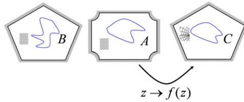
Figure 3. A and B are critical systems defined in different domains. The system C is the image of A under the conformal transformation f(z) which maps domain A onto domain B . Conformal invariance is the statistical identity of B and C .
