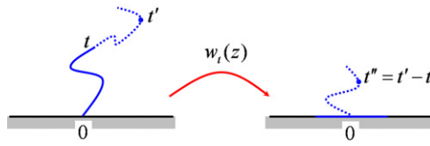
Figure 8. The image of the [t, t'] part of the curve on the left created by the mapping w_t(z) is statistically identical to the [0, t''] part of the same curve on the right.
