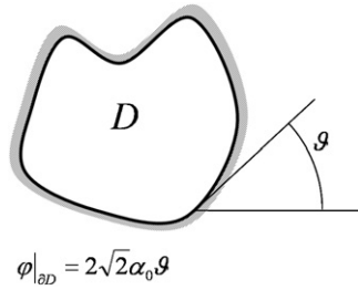
Figure 7. Boundary condition (25). \vartheta = -\arg f'_D|_{\partial D} .
