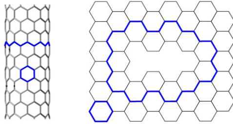
Figure 5. If a loop wraps around the cylinder, the difference between the numbers of left and right turns is 0, otherwise it is \pm 6 . On a flat domain of the same topology—annulus—this difference is \pm 6 for all loops.
