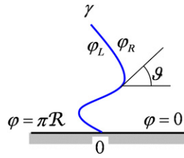
Figure 9. The SLE field \varphi on \gamma measures the winding angle \vartheta (see equation (45)). The tangential component of the current \partial_t \varphi on \gamma measures the curvature.
