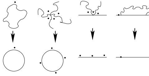
Figure 11. The uniformizing conformal maps for various cases considered. The dots denote that points where the electric field is measured.
