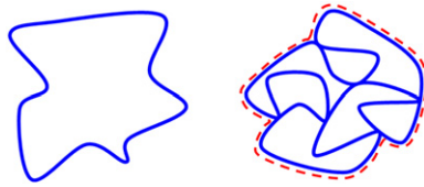
Figure 4. Schematic behaviour of dilute (left) and dense (right) loops. The external perimeter of the dense curve is a dilute curve.
