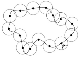
Figure 10. A curve covered by discs.
